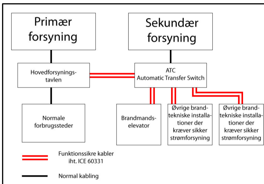
Figur 04.02.01: Diagram for sikker strømforsyning
